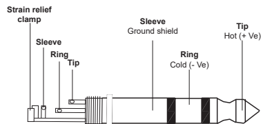
Balanced use of 1/4" jack TRS connector
